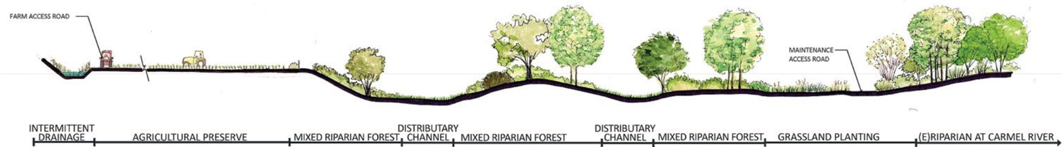
TYPICAL SECTION 1" = 30' horizontal, x 3 vertical
