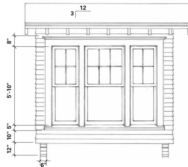
Box Bay Elevation
