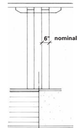
Double Post on Solid Rail
