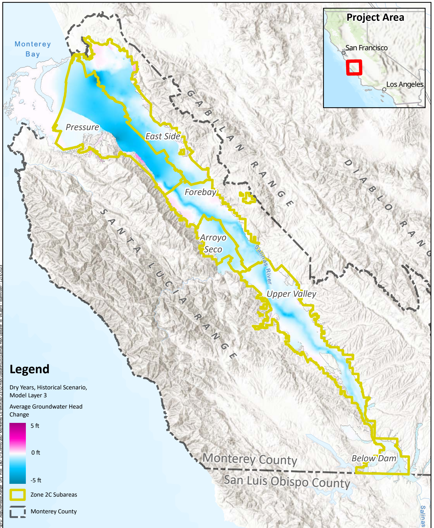
Average Annual Groundwater Head Change Historical Scenario, Dry Years 180-Foot Aquifer & Equivalent
