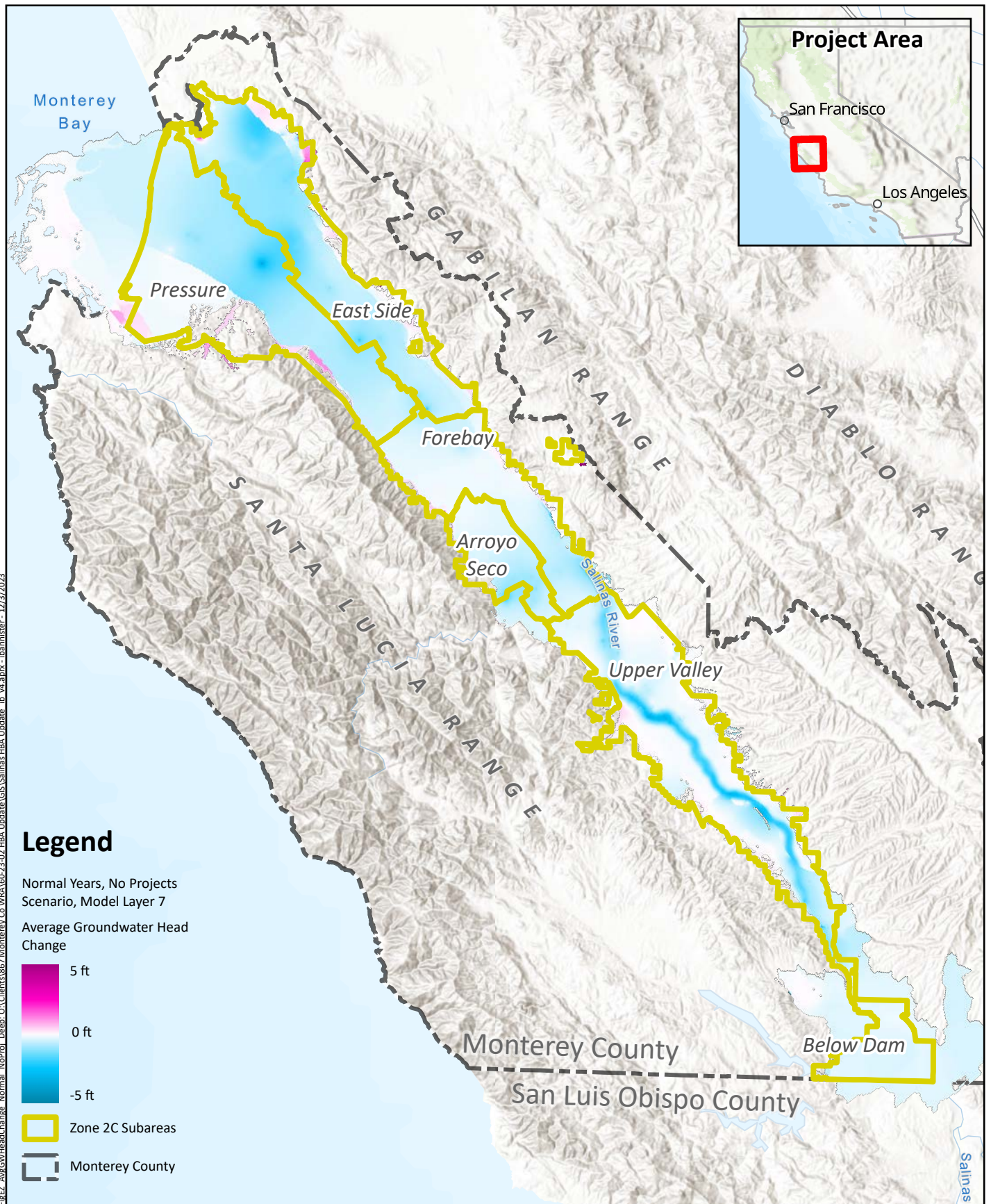
Average Annual Groundwater Head Change, No Projects Scenario, Normal Years Deep Aquifer
