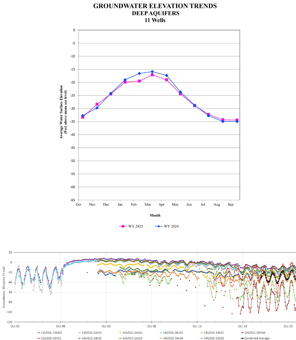
Figure 9: Groundwater Elevation Trends in the Deep Aquifers
