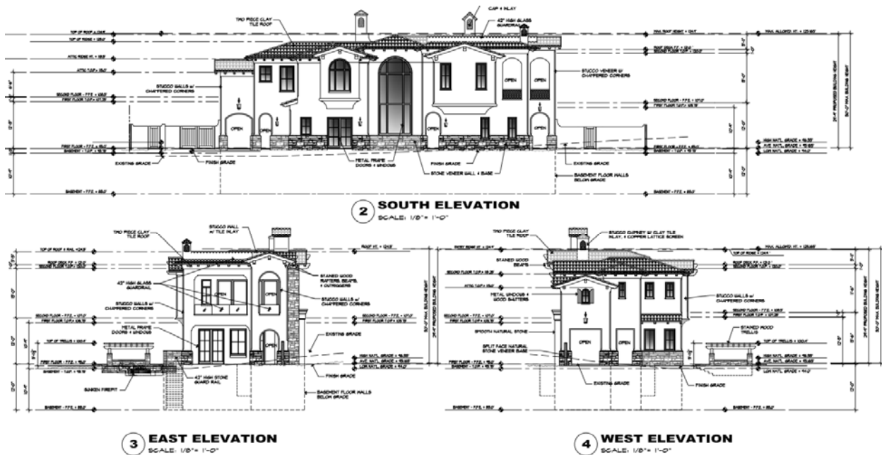
HOUSE ELEVATIONS
