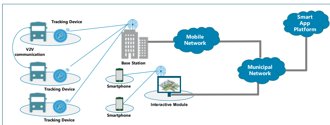
Figure 91. High-level architecture of the Smart Public Transportation application.
