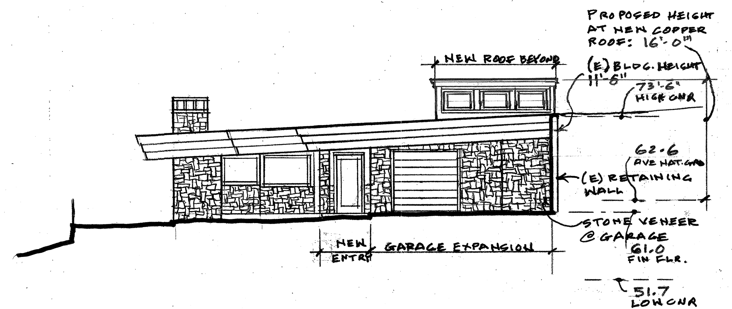
EAST ELEVATION
