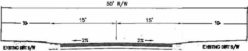
EXISTING COLLEGE STREET - TYP. SECTION
