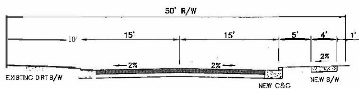
PROPOSED GODCHAUX STREET - TYP. SECTION
