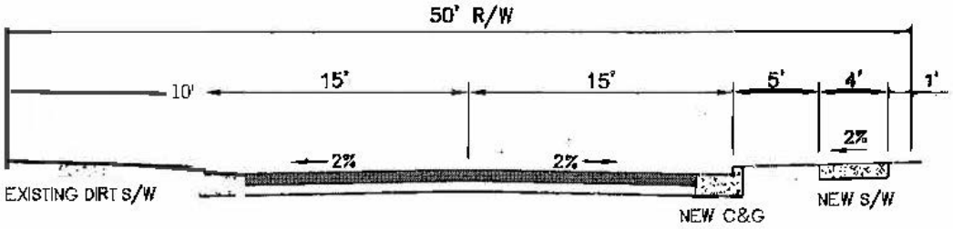
PROPOSED CENTER STREET - TYP. SECTION
