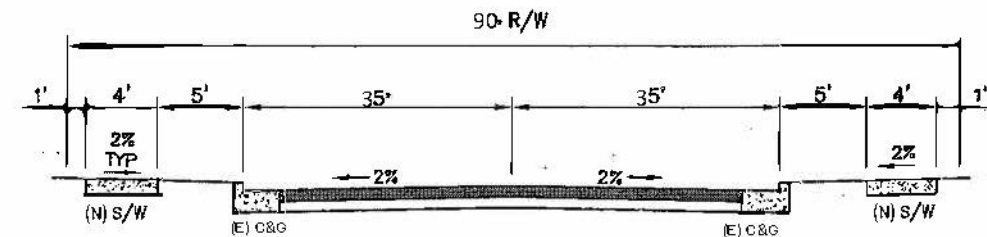
PROPOSED CLAY STREET - TYP. SECTION
