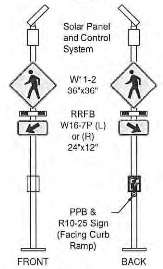
TYPICAL RRFB ASSEMBLY STANDARD CROSSING (DOUBLE SIDED) NTS
