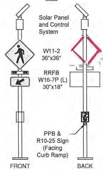
TYPICAL RRFB ASSEMBLY STANDARD CROSSING (SINGLE SIDED) NTS
