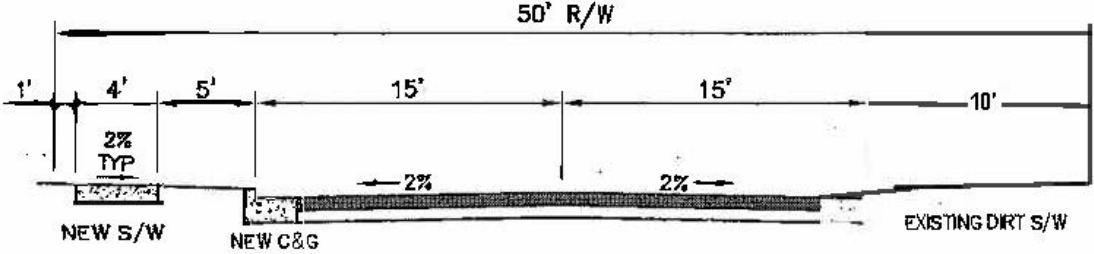
PROPOSED COLLEGE STREET - TYP. SECTION
