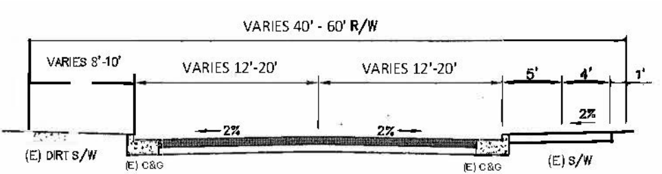
EXISTING CRANE STREET - TYP. SECTION
