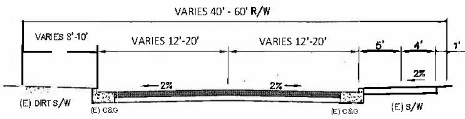
EXISTING PRESTON STREET - TYP. SECTION
