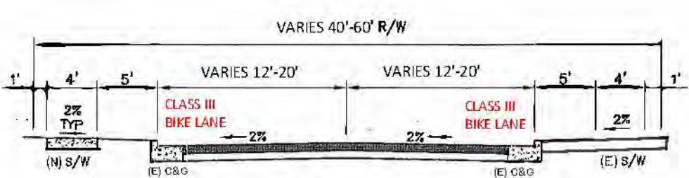
PROPOSED UNION STREET - TYP. SECTION
