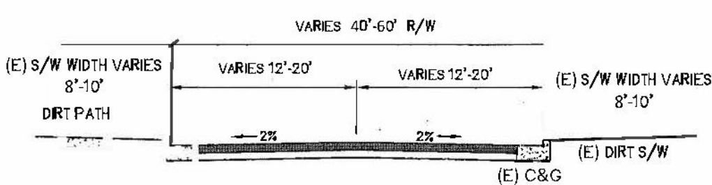
EXISTING UNION STREET - TYP. SECTION
