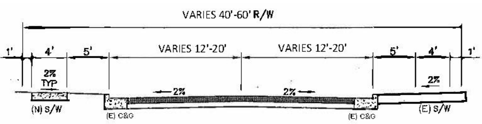
PROPOSED PRESTON STREET - TYP. SECTION
