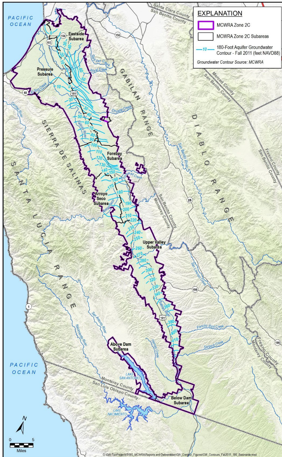
Figure 4-18. Fall 2011 Groundwater Elevation in Basin Fill Aquifer, 180-Foot Aquifer, and Shallow Zone of the Eastside Subarea
