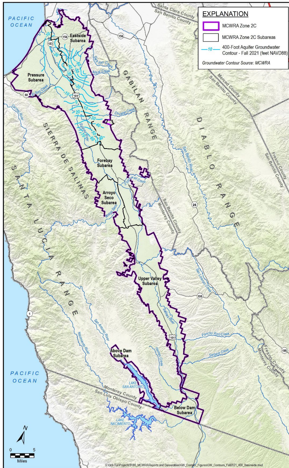
Figure 4-22. Fall 2021 Groundwater Elevation in 400-Foot Aquifer and Deep Zone of the Eastside Subarea
