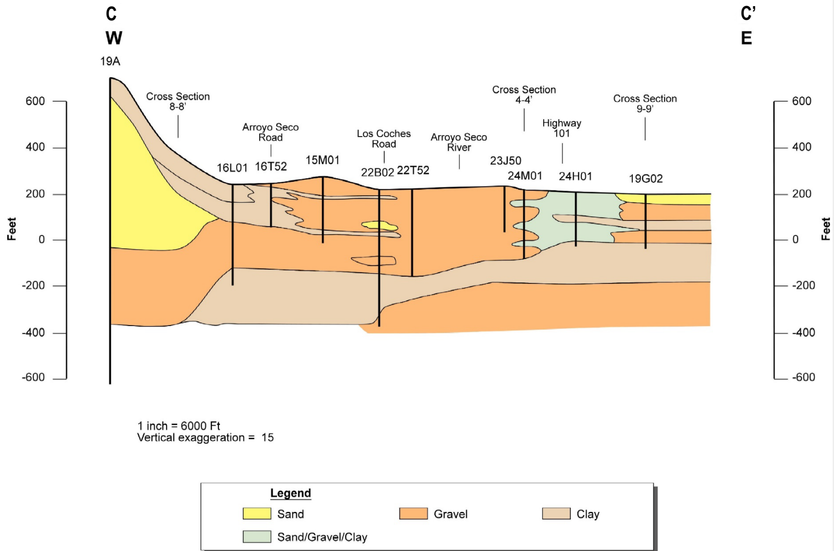
Figure 2-6. Cross Section C-C' (adapted from section 5-5' Staal, Gardner, & Dunne Inc, 1994)
