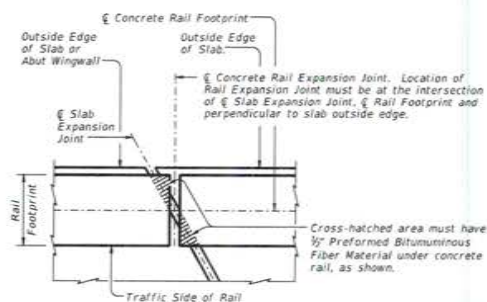
PLAN OF RAIL AT EXPANSION JOINTS
