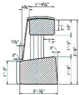
TYPE 86H SECTION
