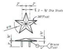
BRONZE STAR DETAIL ©
