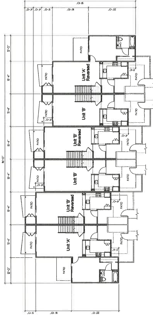
FIRST FLOOR Floor Area = 3630 s.f.
