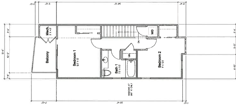
UNITS 'A' & 'B' SECOND FLOOR PLAN 681 S.F.
