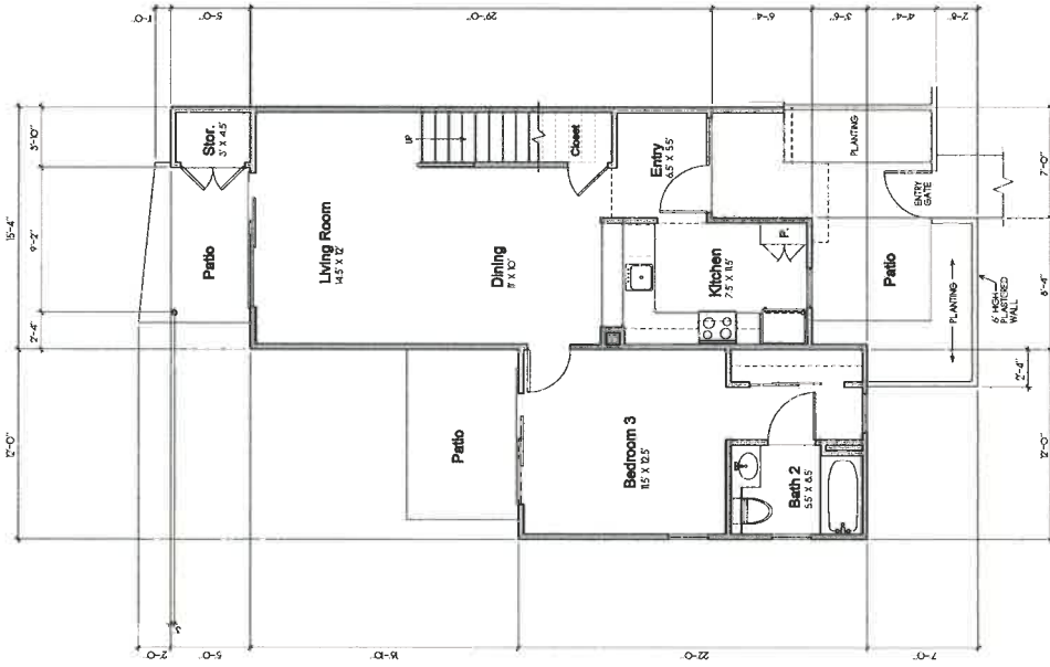
UNIT 'A' FIRST FLOOR PLAN 782 S.F.
