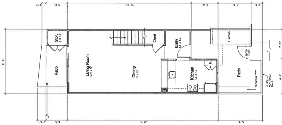
UNIT 'B' FIRST FLOOR PLAN 817 S.F.
