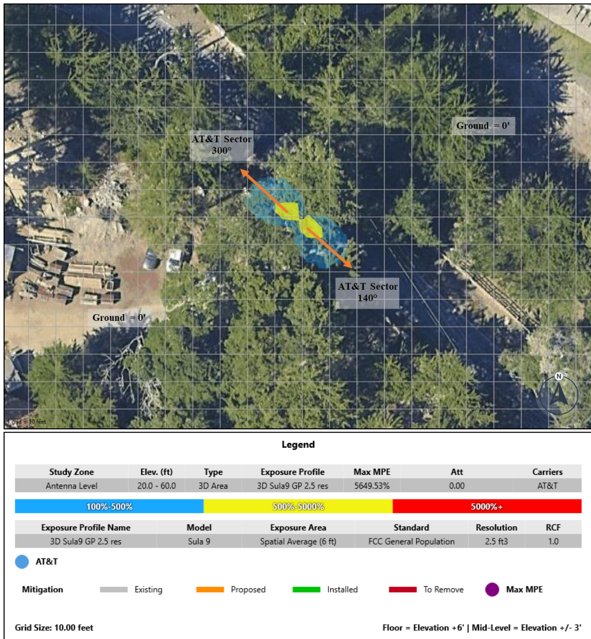
Figure1.1: Antenna Level
