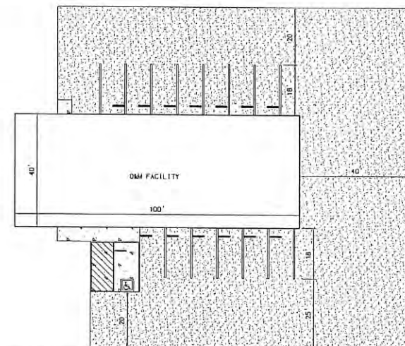
PLAN VIEW OF O&M FACILITY AND PARKING AREA NOT TO SCALE
