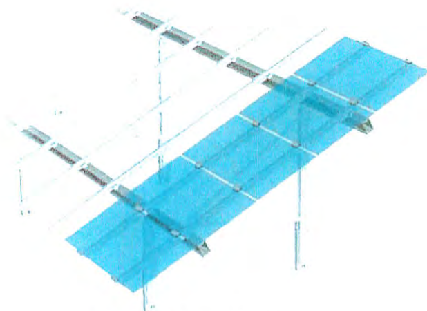
Photo 3. Fixed-tilt racking system
