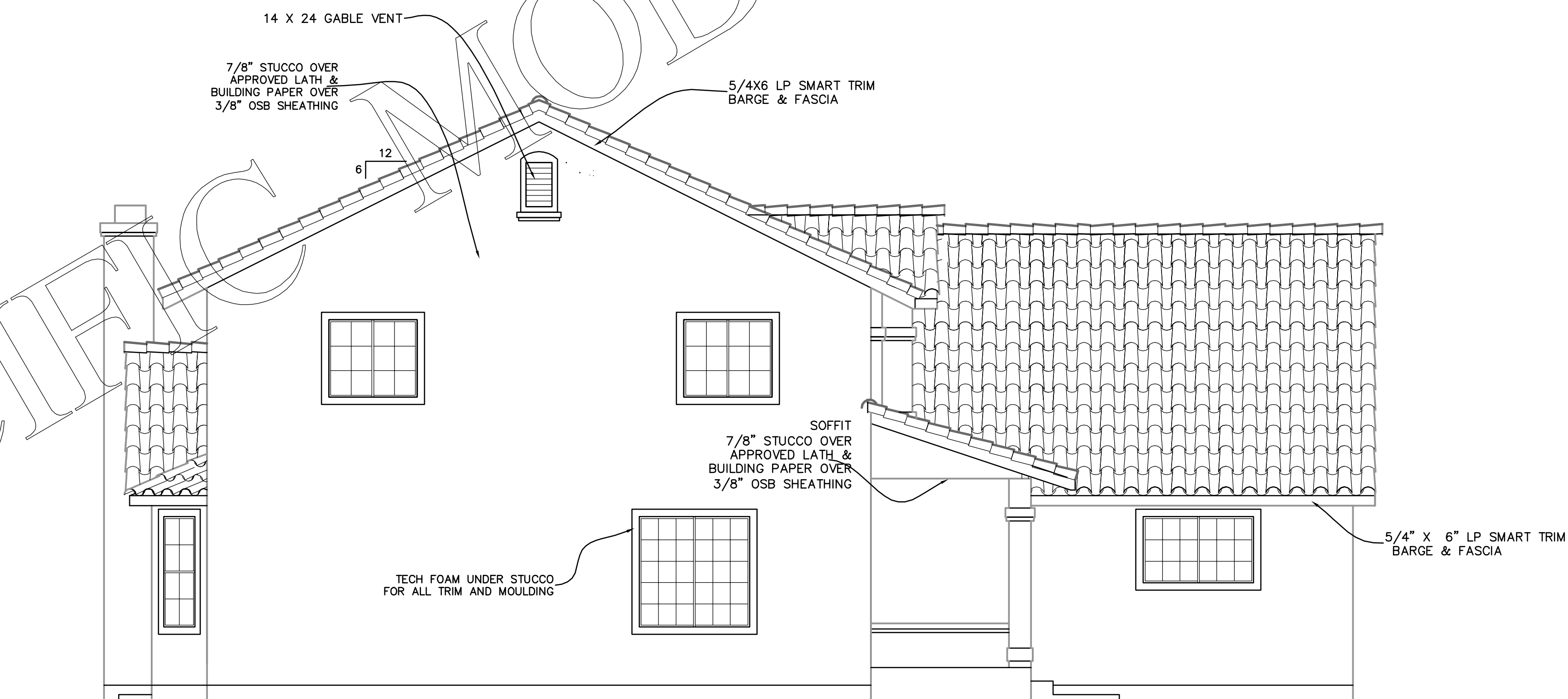
LEFT ELEVATION
