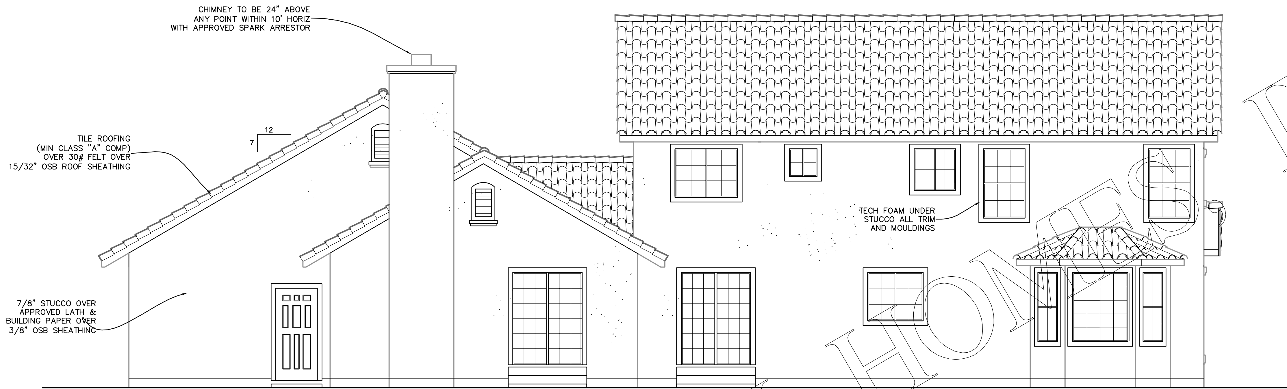
BACK ELEVATION
