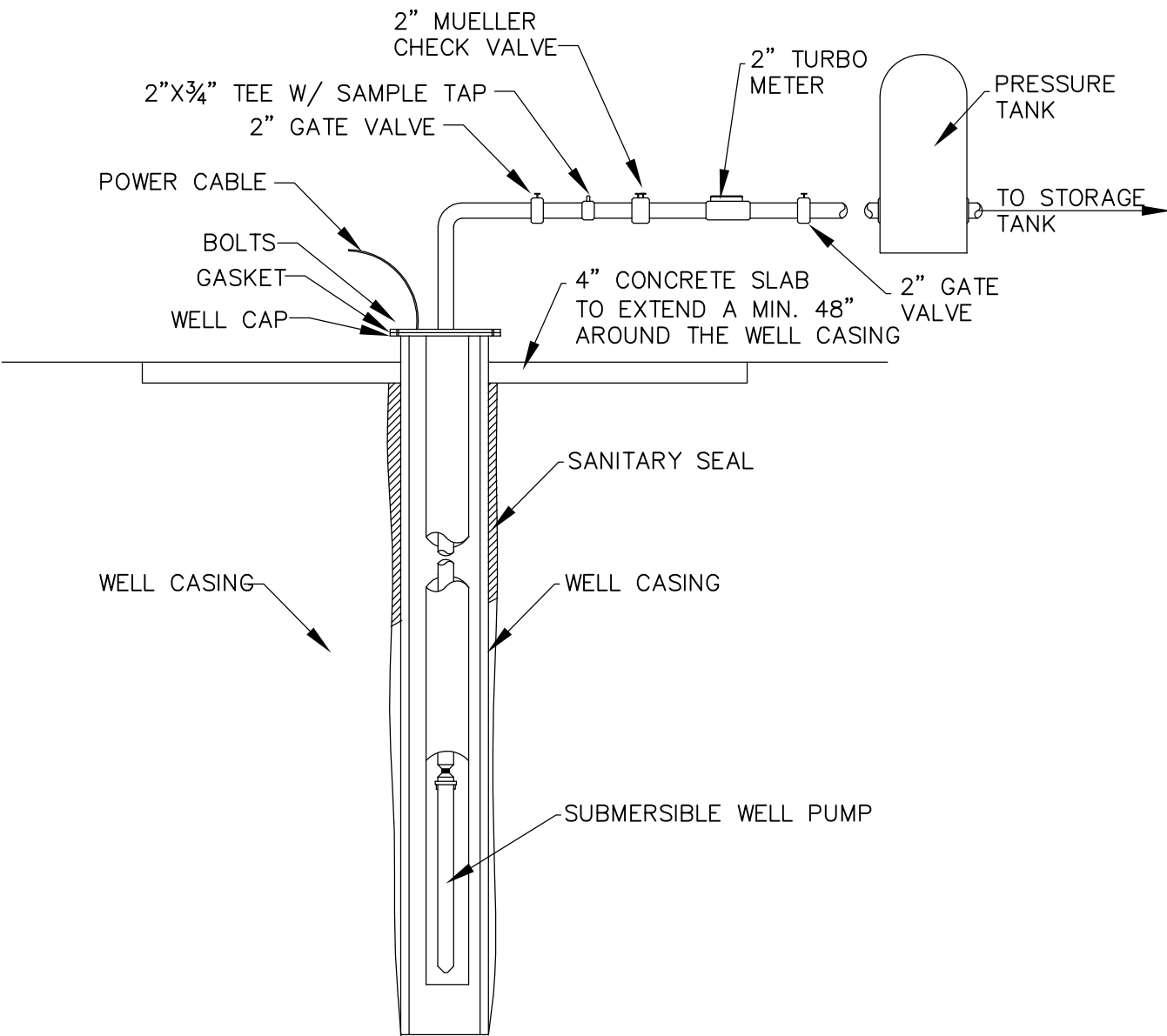
WELLHEAD DETAIL NOT TO SCALE
