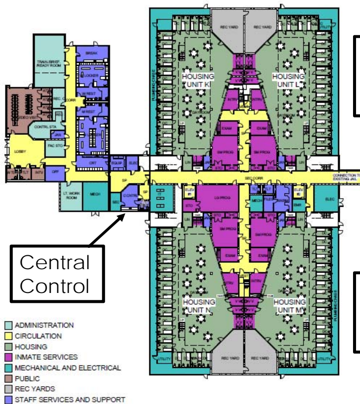
1 HOUSING FLOOR PLAN - LEVEL 1
