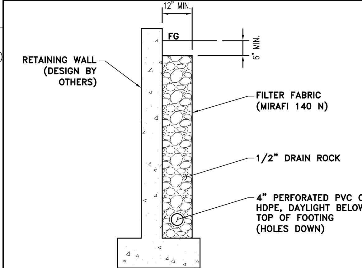
C C3 RET. WALL SUBDRAIN NTS
