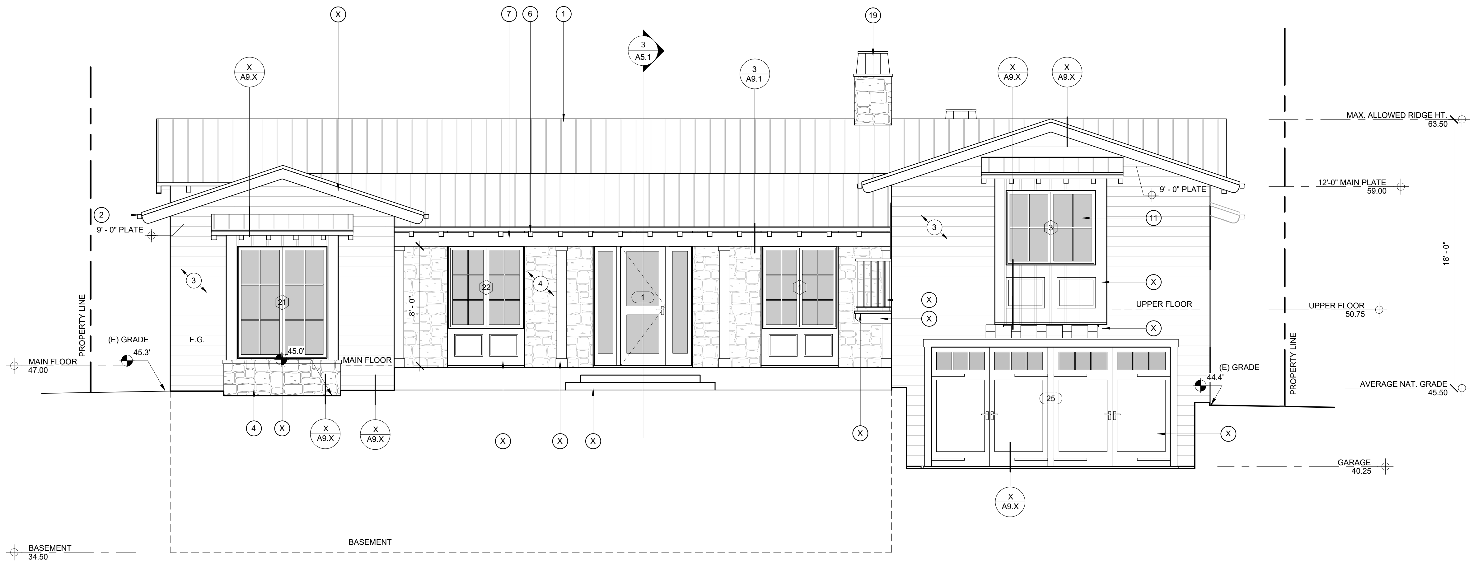
EAST ELEVATION
