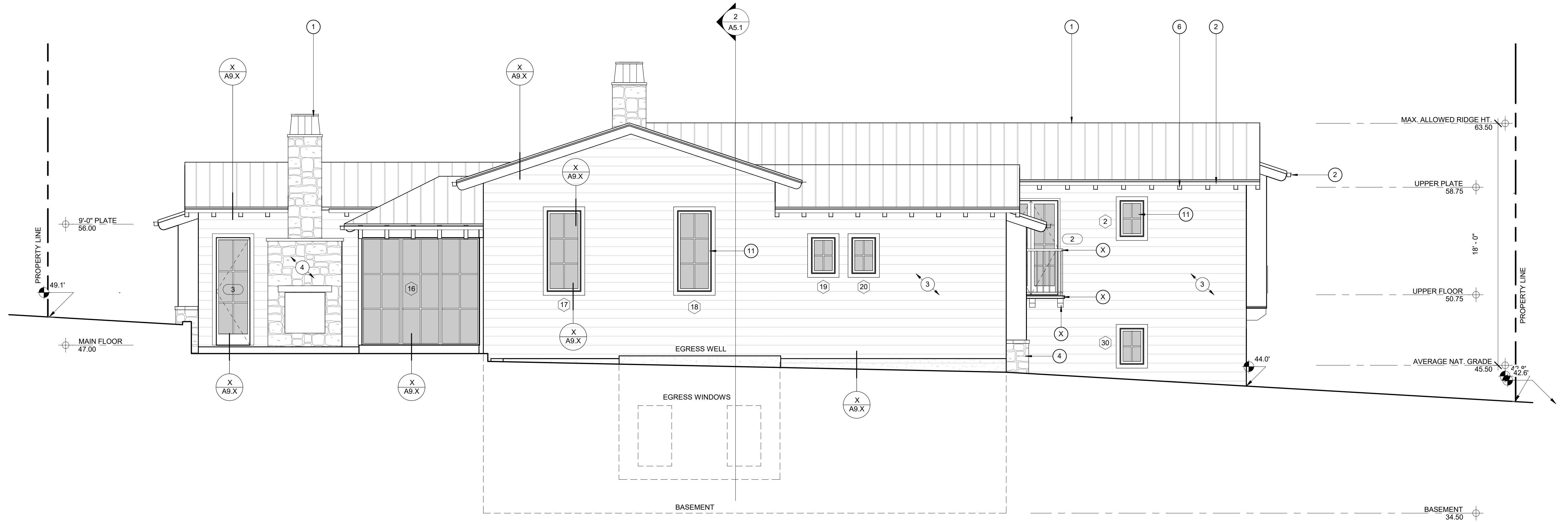
NORTH ELEVATION
