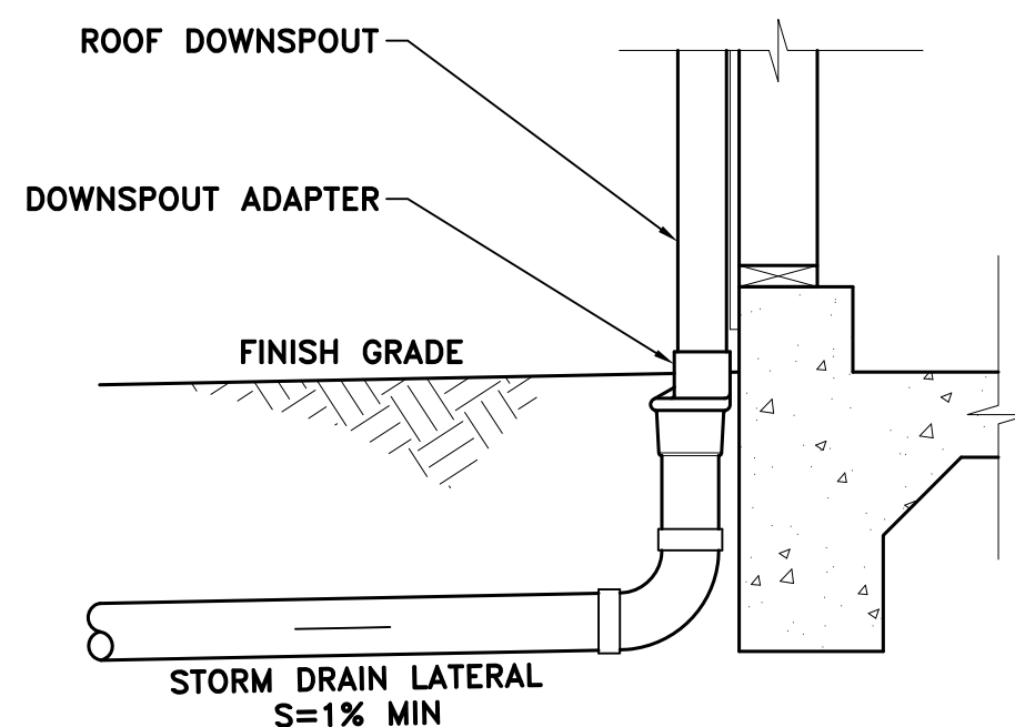
F C3 ROOF DRAIN CONNECTION NTS
