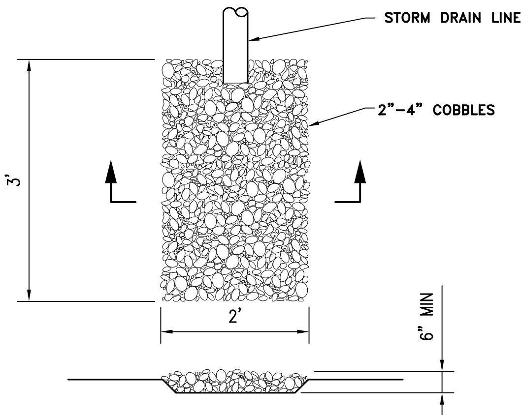
H C3 ENERGY DISSIPATER NTS
