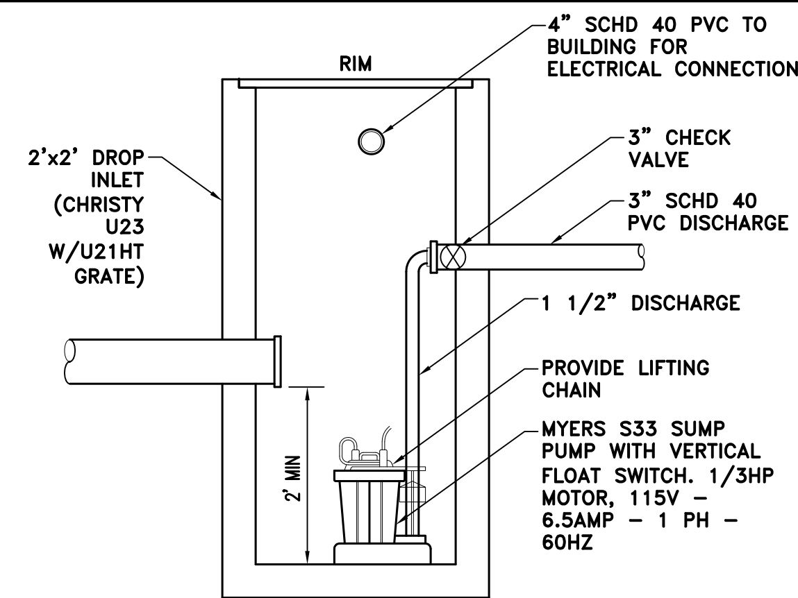
E C3 C.B. W/PUMP NTS
