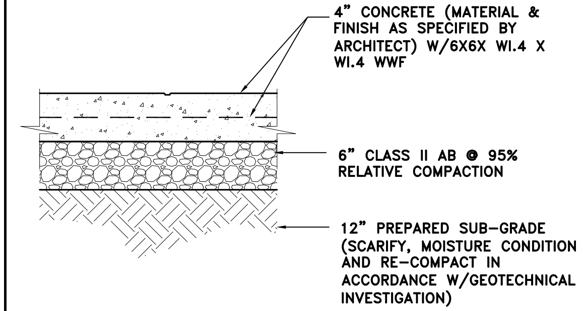
A C3 CONCRETE PAVEMENT NTS
