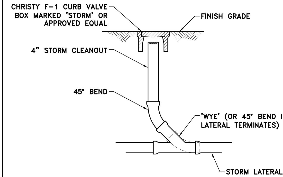
D C3 CLEAN-OUT @ GRADE NTS
