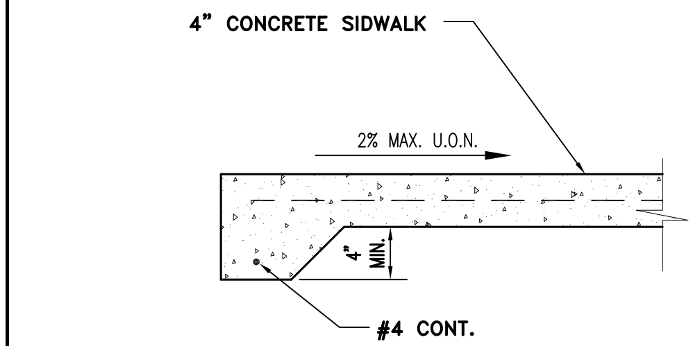
B C3 THICKENED EDGE NTS
