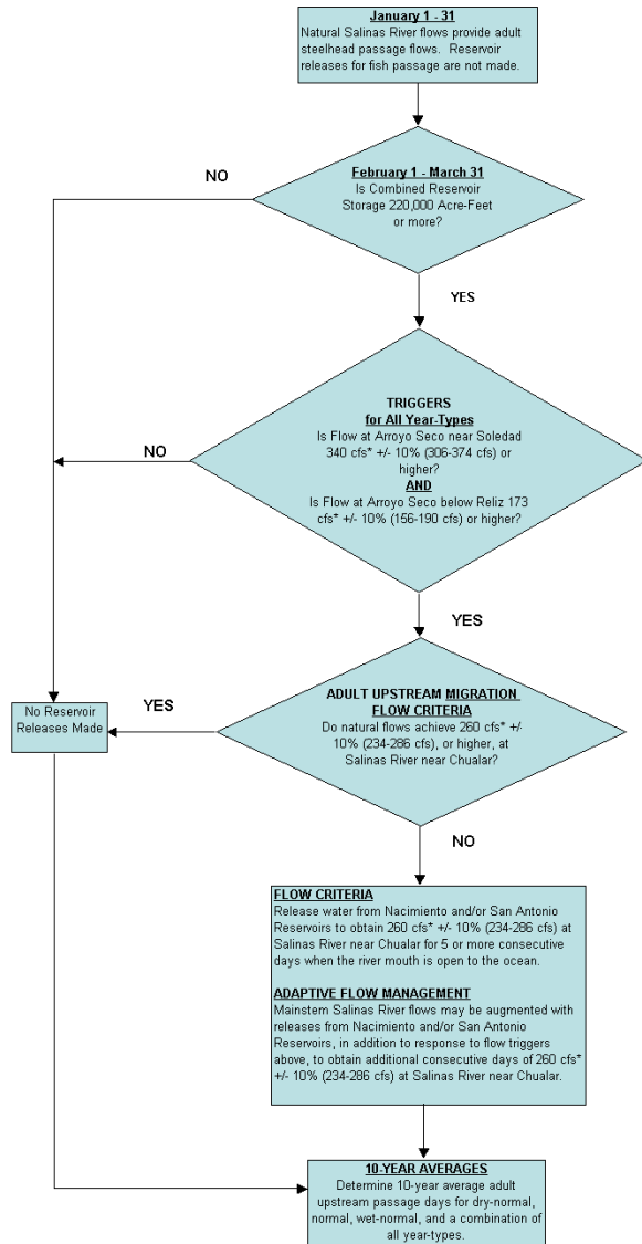
Figure 3. Adult Upstream Migration Action Flow Chart
