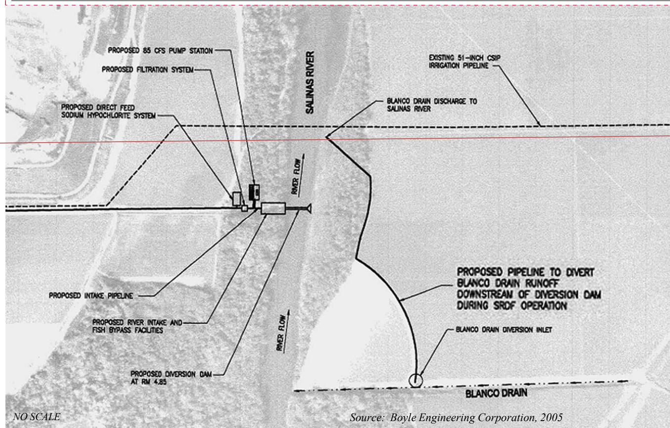
Figure 7. Blanco Drain Diversion Pipeline Proposed Location
