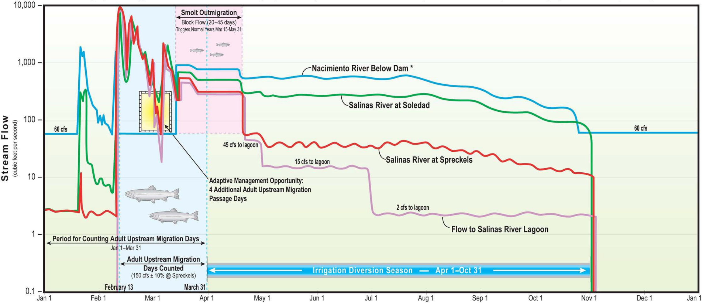
Figure 9. Illustrative Example of Salinas Valley Water Project Stream Flows
