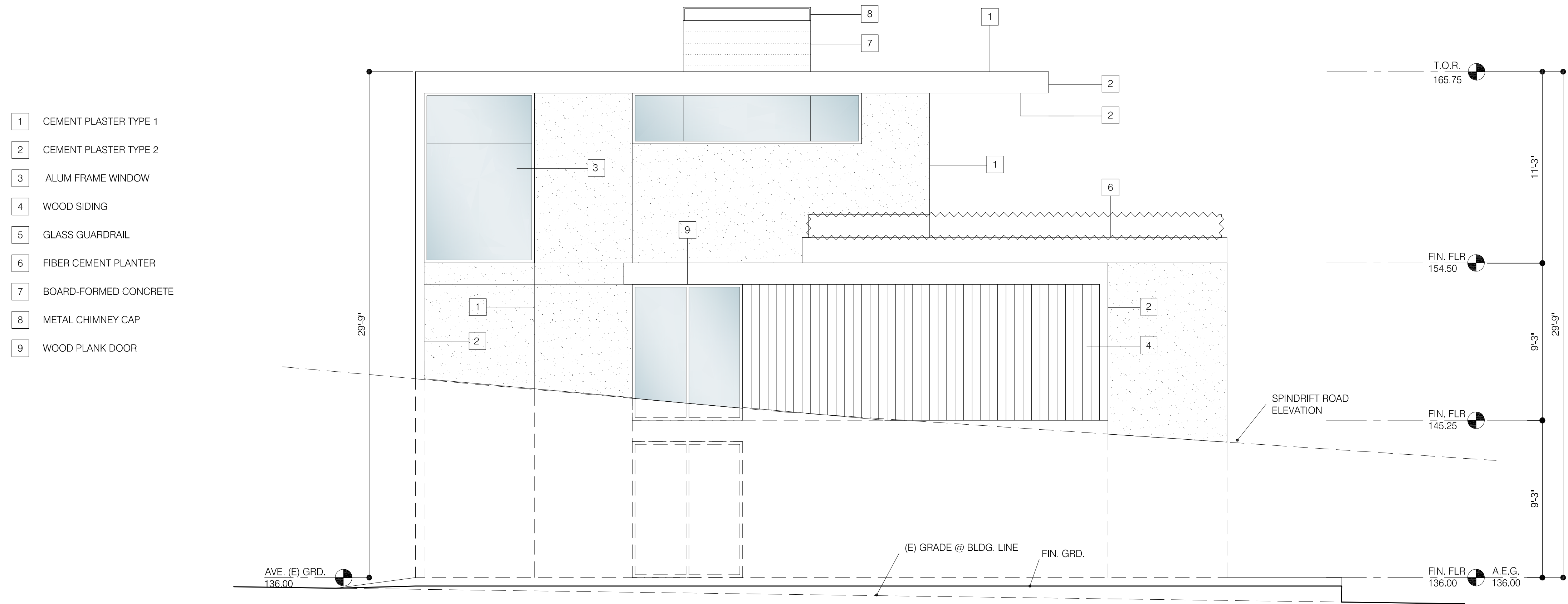
NORTH ELEVATION 1/4" = 1'-0"
