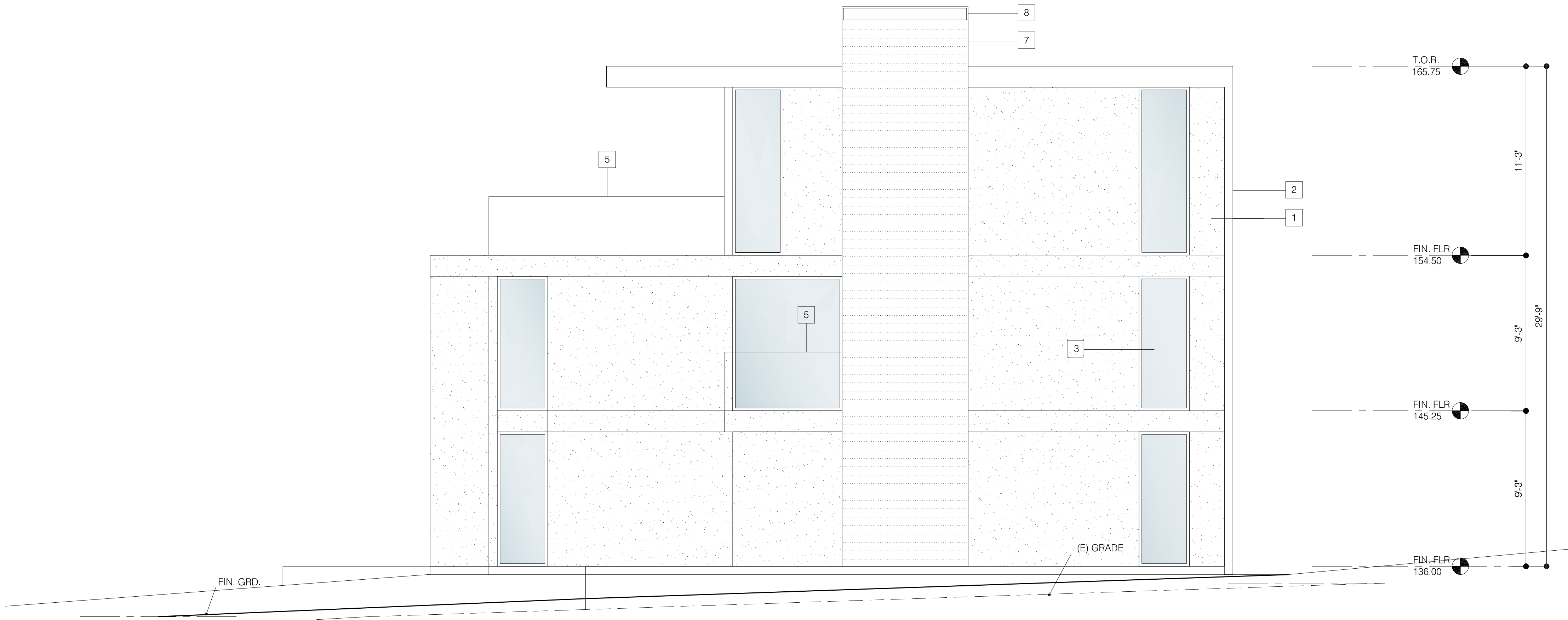
SOUTH ELEVATION 1/4" = 1'-0"
