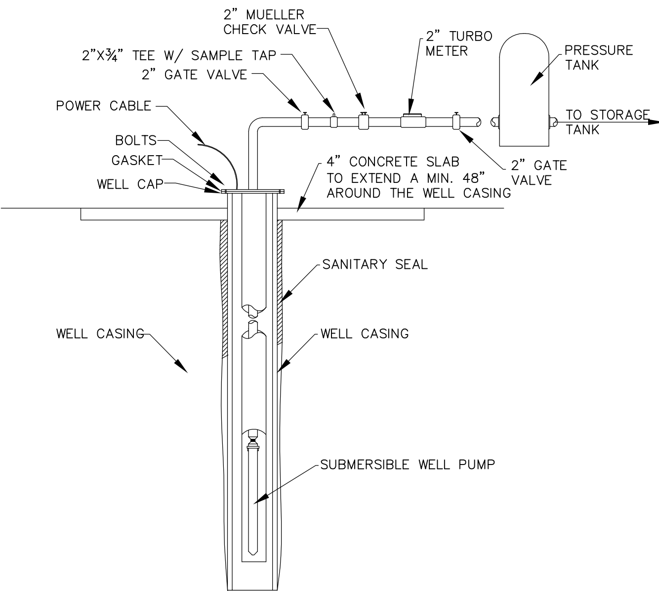
WELLHEAD DETAIL 2 NOT TO SCALE
