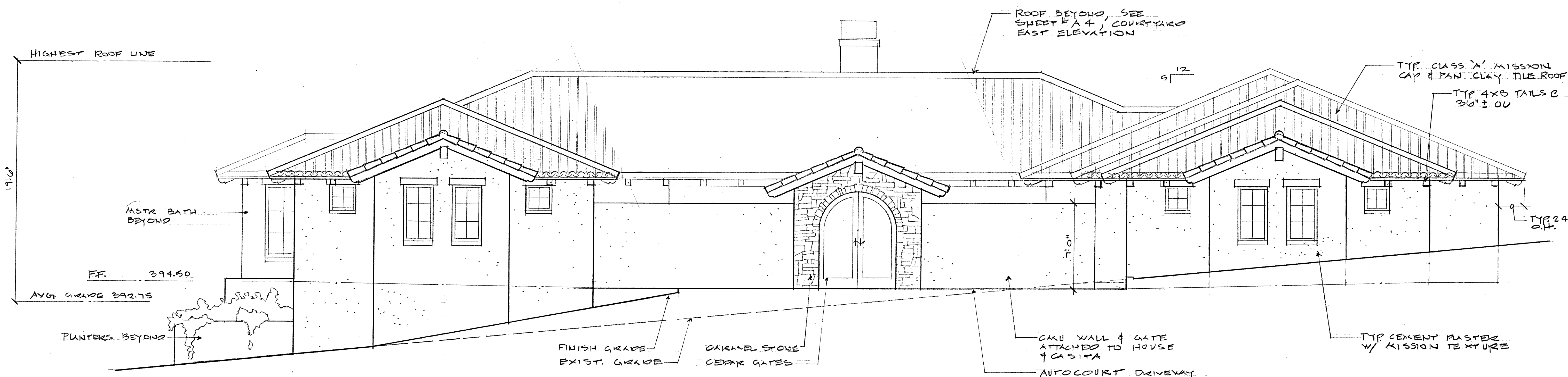
EAST ELEVATION
