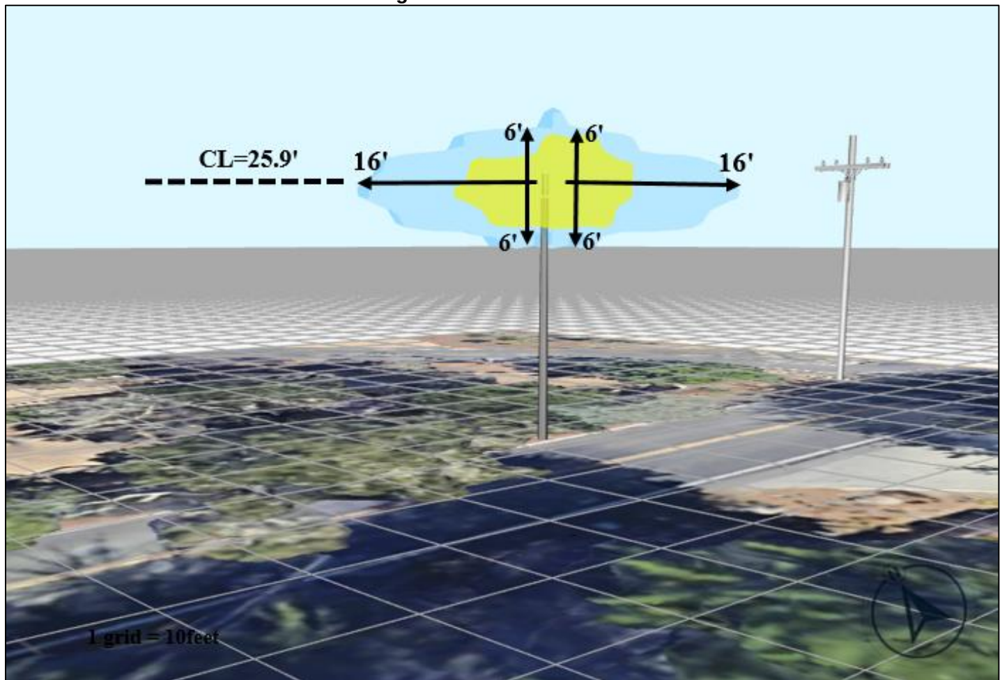
Figure 1.3: Ground Level.
