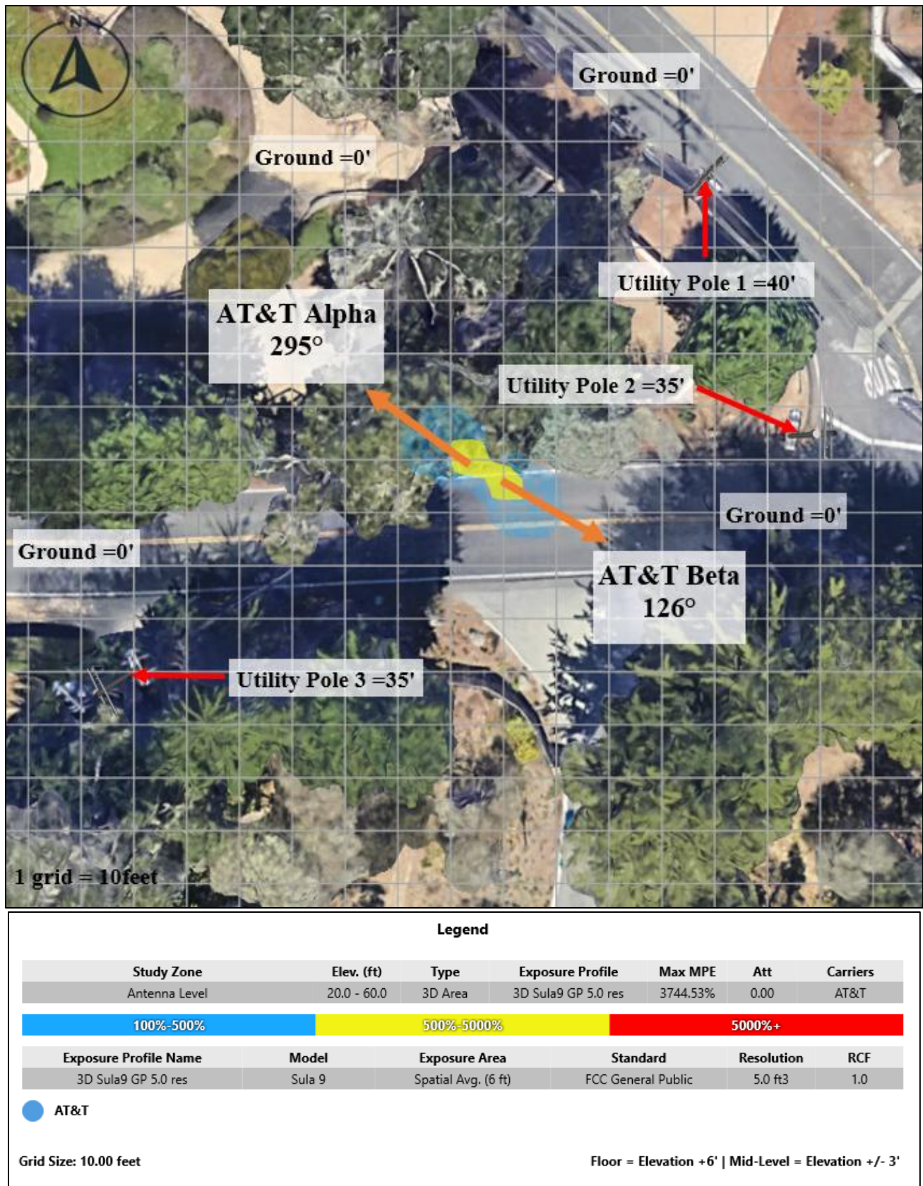
Figure1.1: Antenna Level
