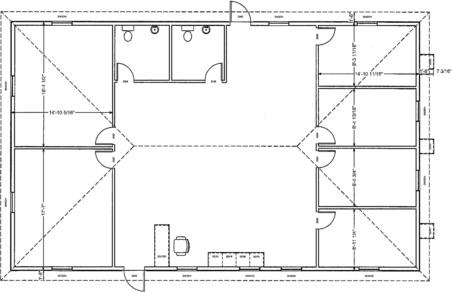
36x60 Conceptual floor plan
