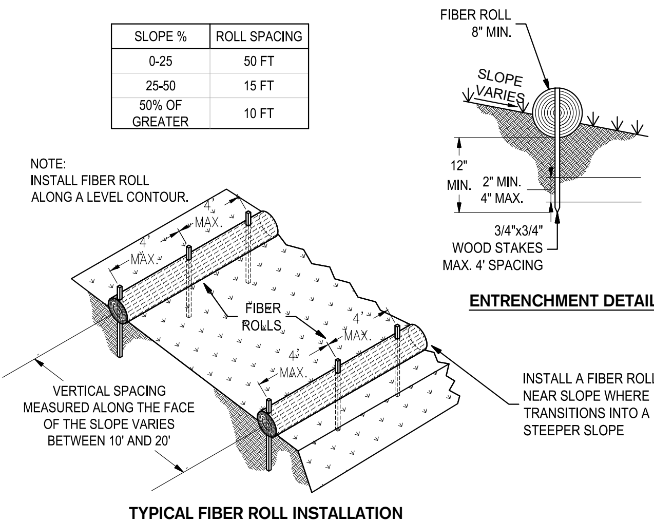
3 FIBER ROLLS (SE-5) SCALE: NTS
