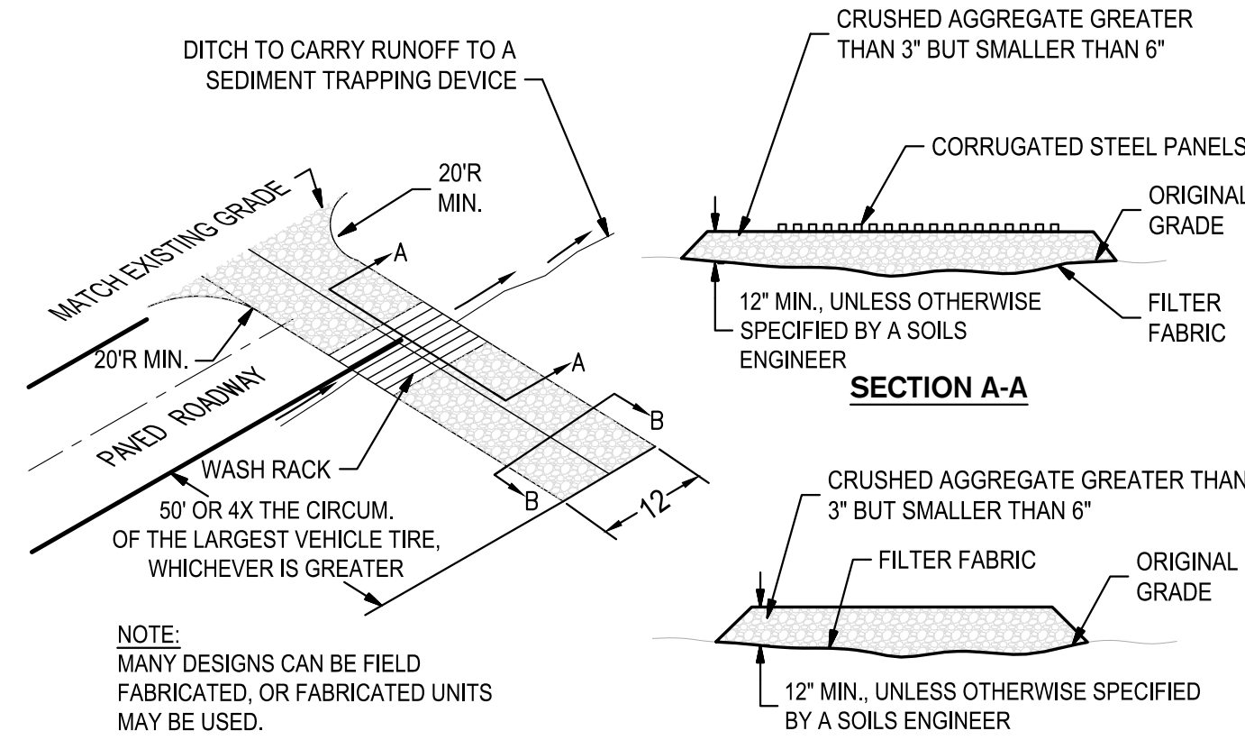
4 STABILIZED CONSTRUCTION ENTRANCE/EXIT TIRE WASH (TC-1) SCALE: NTS
