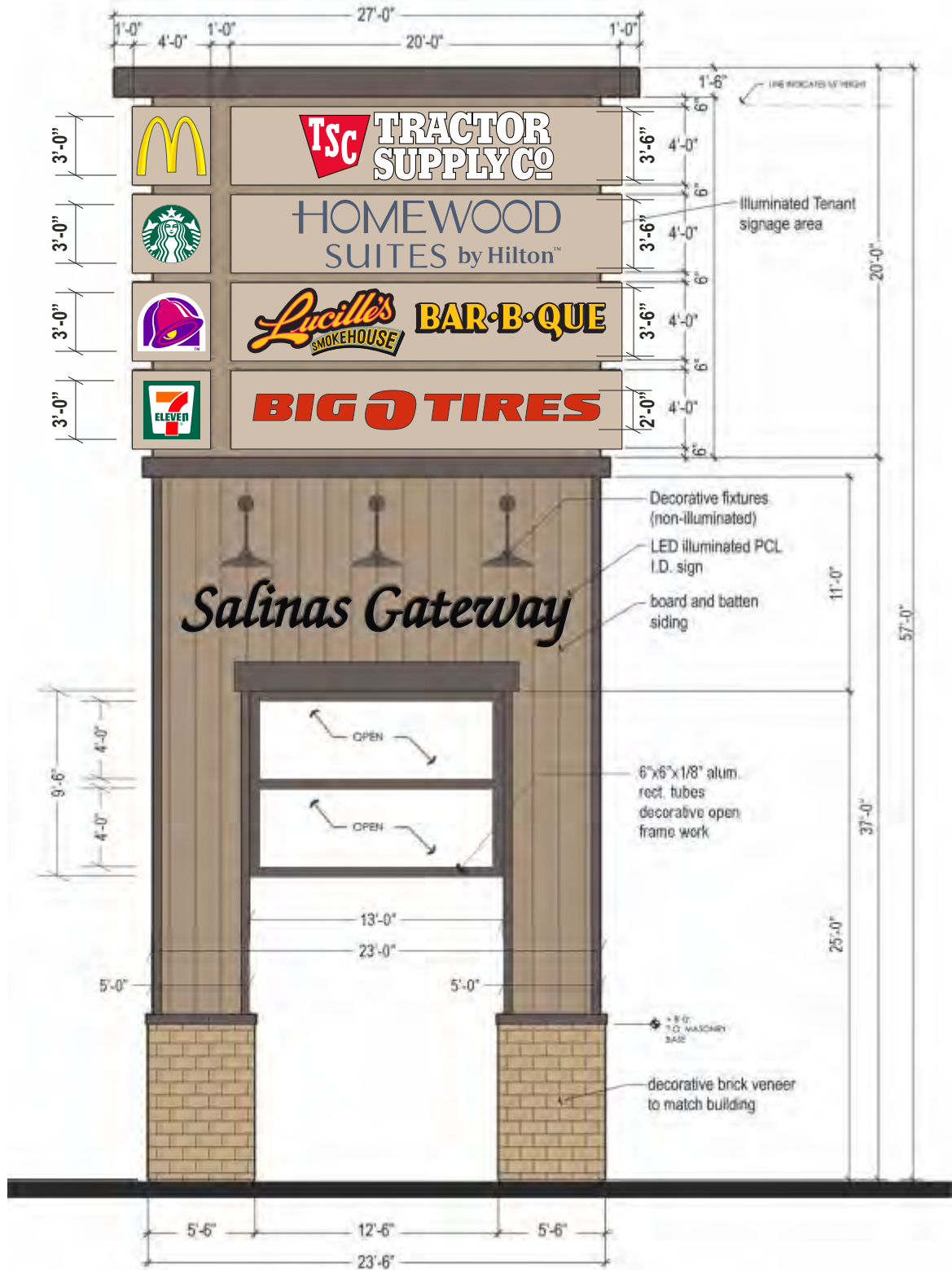
D/F LED ILLUMINATED PYLON SIGN Scale: 1/8" = 1'-0"
