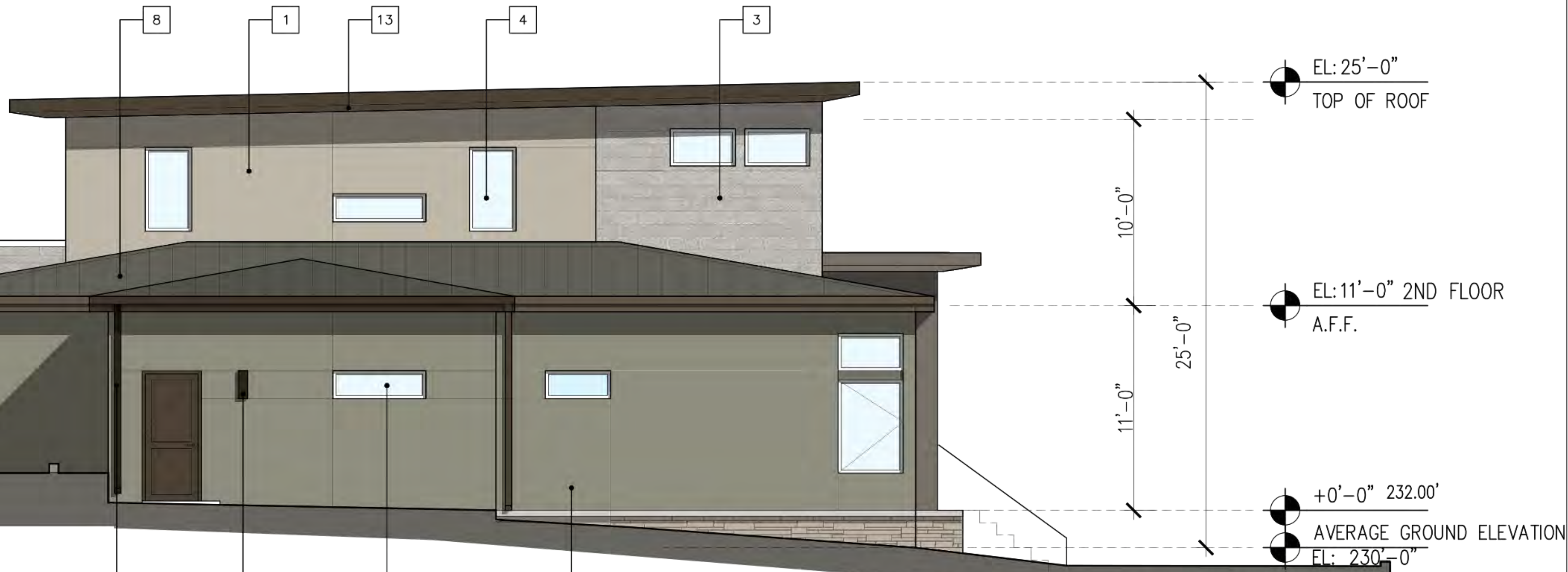
2 EAST SIDE ELEVATION SCALE: 1/4" = 1'
