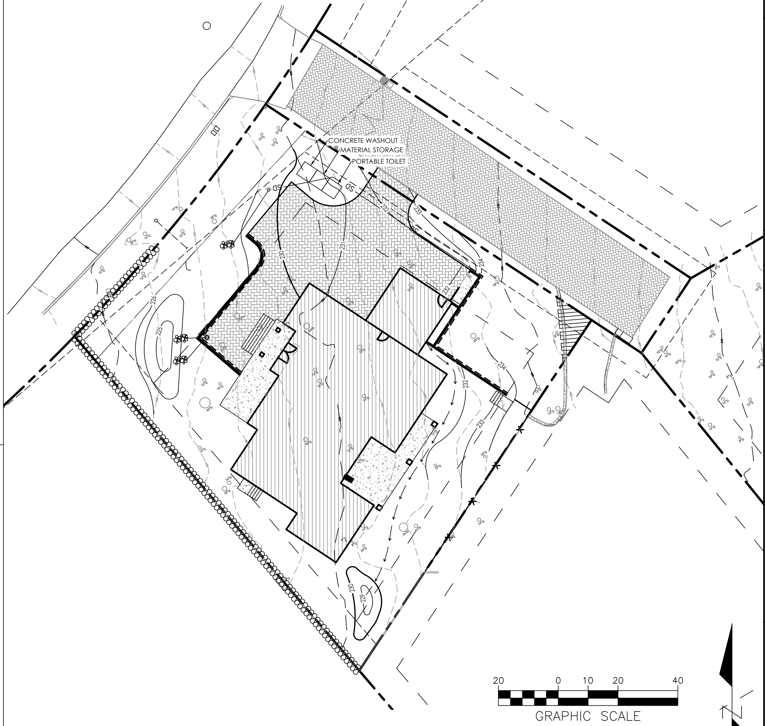
A C4 EROSION CONTROL PLAN SCALE: 1"=20'
