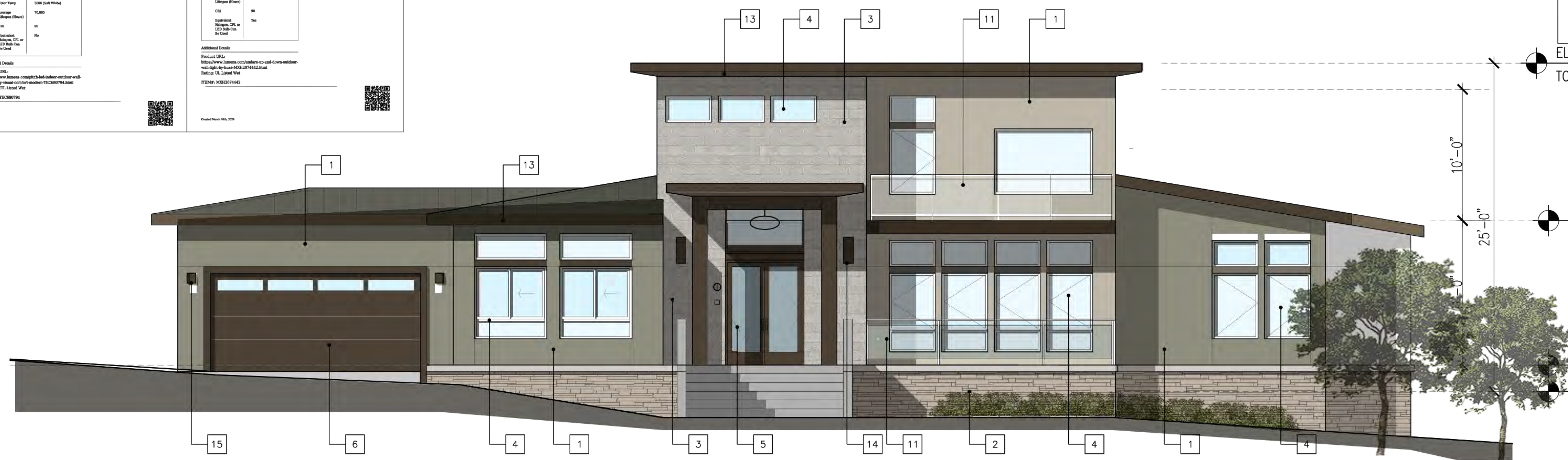
1 FRONT ELEVATION SCALE: 1/4" = 1'
