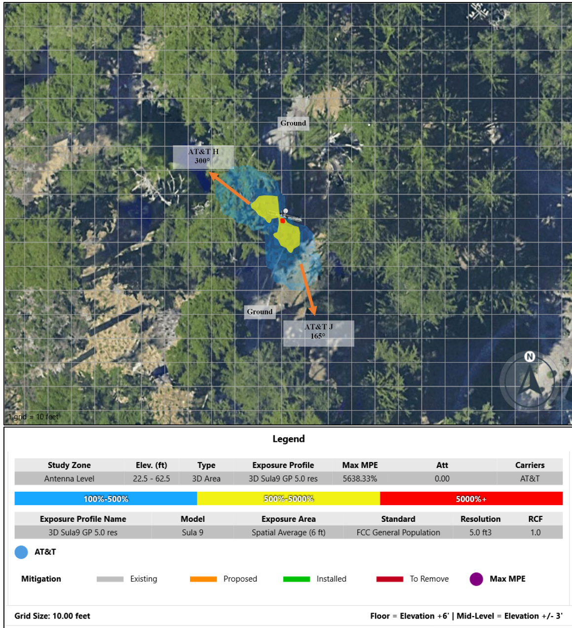
Figure1.1: Antenna Level
