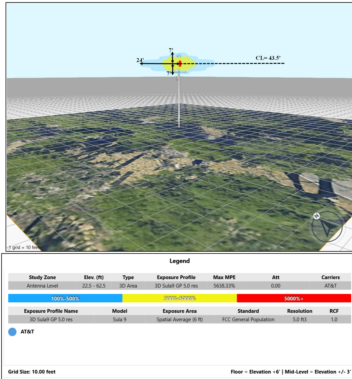
Figure1.3: Elevation Level
