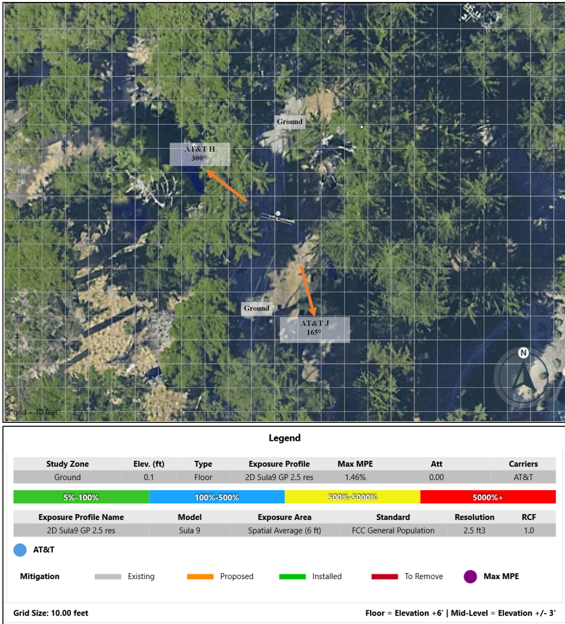
Figure 1.2: Ground Level.
