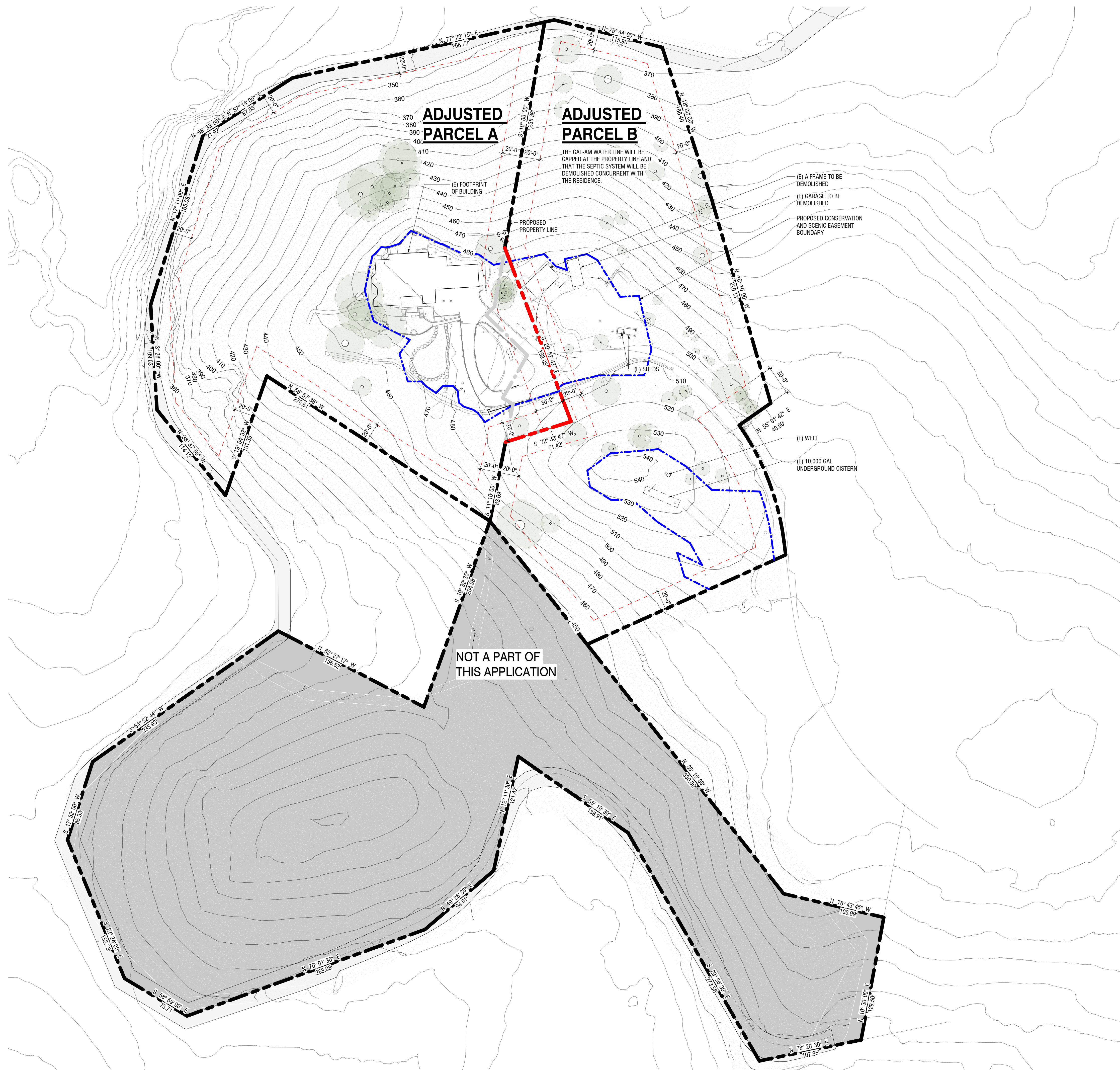
1 PROPOSED SITE PLAN LLA 1" = 50'-0"
